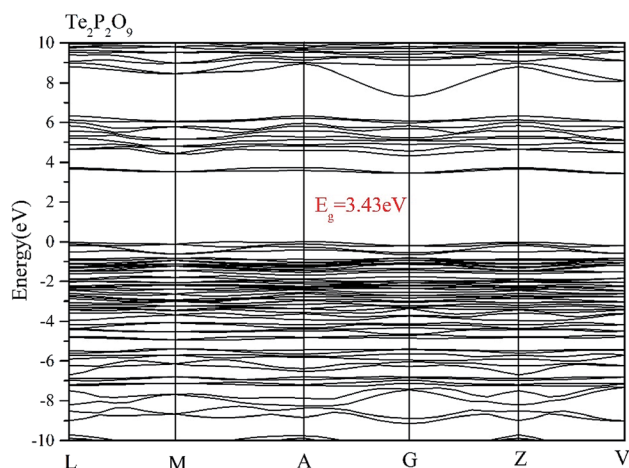
Fig. 1 Obtained band structures of \text{Te}_2\text{P}_2\text{O}_9 .
