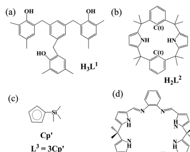
Chart 1 Ligand structures of (a) tris(alkyloxi)arene, (b) trans -calix[2]pyrrole[2]benzene, (c) silylcyclopentadiene, and (d) octadentate Schiff-base polypyrrolic macrocycle.
