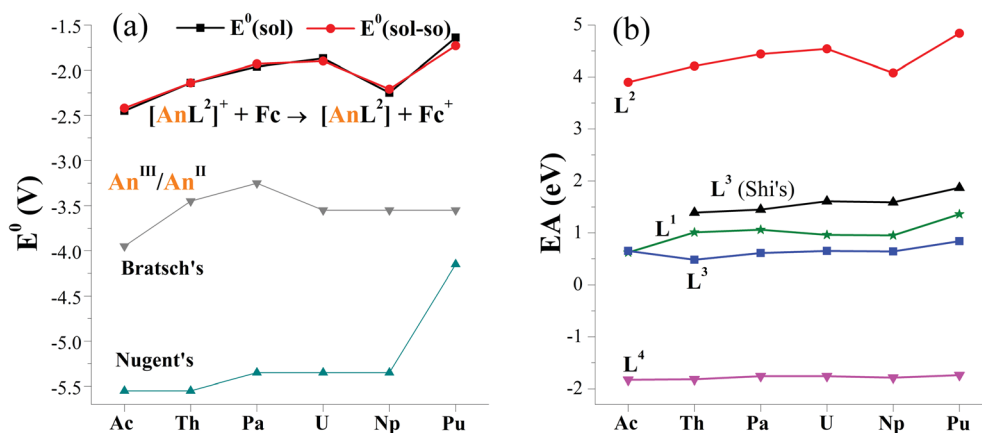
Fig. 2 (a) Reduction potentials ( E^0 in V) of [\text{AnL}^{2+}]/[\text{AnL}^2] (An = Ac–Pu) versus \text{Fc}^+/\text{Fc} in THF, along with previously reported values for \text{An}^{\text{III}}/\text{An}^{\text{II}} . 26,27 Noting that the solvation energy is included in E^0(\text{sol}) while additional spin–orbit coupling energy in E^0(\text{sol-so}) . (b) Calculated electron affinity (EA) of actinide complexes with various ligands ( L^n , n = 1-4 ), where those of L^3 in THF come from Shi's ref. 31.
