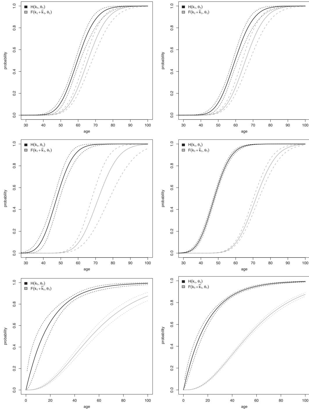
Figure 2. Results of the simulation study with m = 500 families. Top: scenario 1 ( k_1 = 50 , \tilde{k}_1 = 5 , \theta_1 = 1.2 ). Middle: scenario 2 ( k_1 = 40 , \tilde{k}_1 = 20 , \theta_1 = 1.2 ). Bottom: scenario 3 ( k_1 = 1 , \tilde{k}_1 = 2 , \theta_1 = 20 ). Left panels: small families ( n_j \in \{1, 2, 3, 4\} ). Right panels: large families ( n_j \in \{3, 6, 9, 12\} ). Solid black and gray lines are the true distribution functions H_{(k_1, \theta_1)} and F_{(k_1 + \tilde{k}_1, \theta_1)} , respectively. Dashed lines form a band based on estimated pointwise 2.5 and 97.5% percentiles based on M = 1000 Monte Carlo trials.
