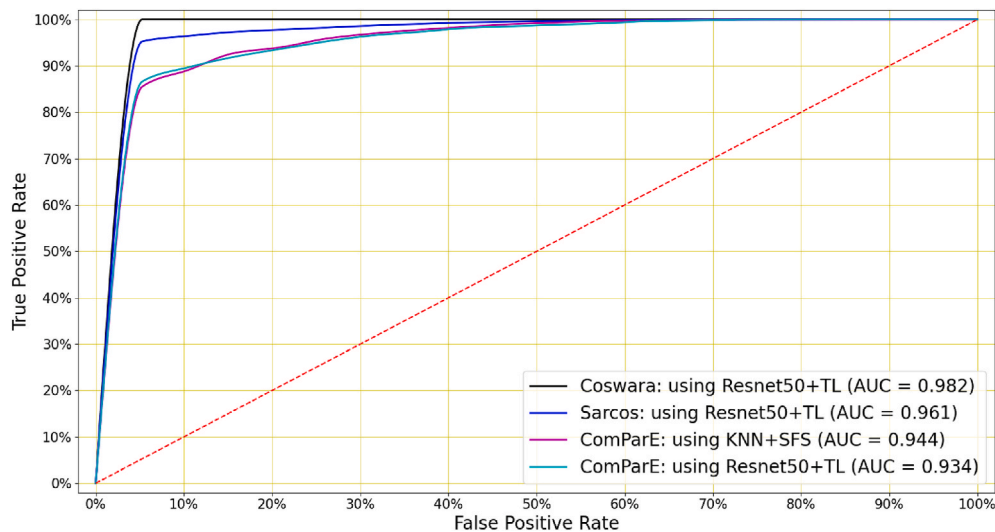
Fig. 5. COVID-19 cough classification: A Resnet50 classifier with transfer learning achieved the highest AUC in classifying COVID-19 coughs for the Coswara and Sarcos datasets (0.982 and 0.961 respectively). For the ComParE dataset, AUCs of 0.944 and 0.934 were achieved by a KNN classifier using 12 features identified by SFS and by a Resnet50 classifier trained by transfer learning respectively.
