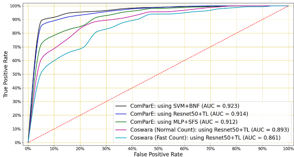
Fig. 7. COVID-19 speech classification: An SVM classifier using bottleneck features (BNF) achieved the highest AUC of 0.923 when classifying COVID-19 speech in ComParE dataset. A Resnet50 trained by transfer learning achieves a slightly lower AUC of 0.914. Speech (normal and fast) in the Coswara dataset can be used to classify COVID-19 with AUCs of 0.893 and 0.861 respectively using a Resnet50 trained by transfer learning.
