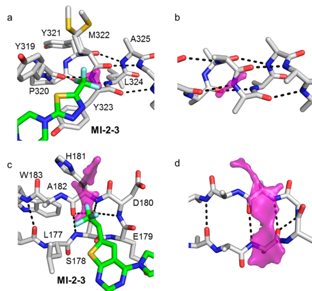
Figure 6. FMAP predictions for \alpha -helix and \beta -sheet structures. (a) Details of the interaction of CF 3 group in MI-2-3 with \alpha -helical fragment in menin and FMAP prediction. (b) FMAP prediction for idealized \alpha -helix for a single peptide bond. Orientation of the \alpha -helix is similar as in panel a. (c) Details of the interaction of CF 3 group in MI-2-3 with \beta -sheet in menin. (d) FMAP prediction for idealized \beta -sheet structure shown in similar orientation as in panel c.
