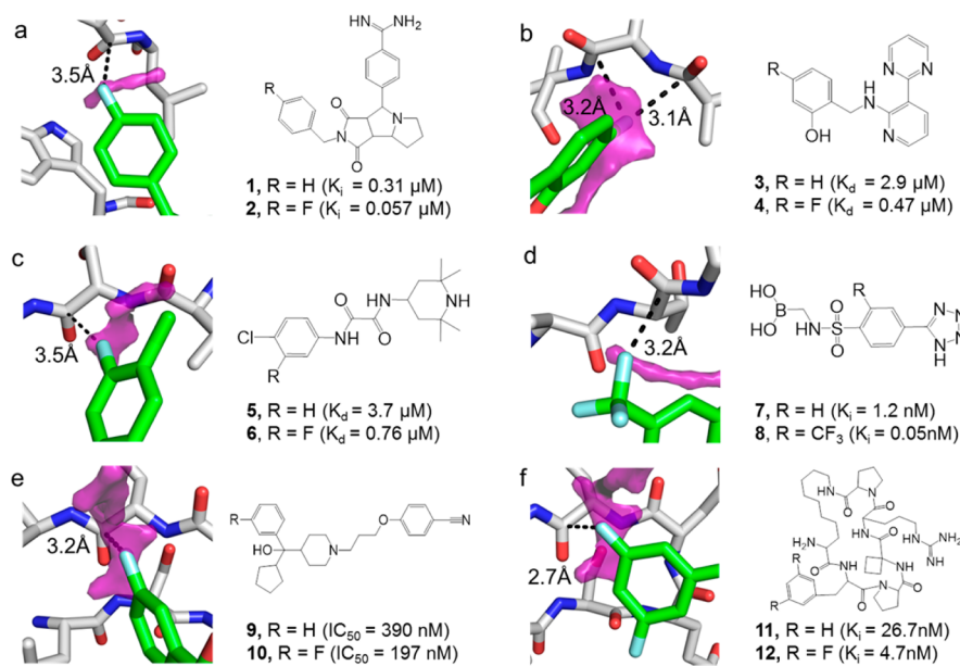
Figure 5. Analysis of FMAP calculations for known inhibitors containing fluorine atoms. Crystal structure of protein–inhibitor complexes showing close C–F...C=O contacts and FMAP predictions (in purple). The structures of inhibitors and activities are also reported. (a) thrombin inhibitor (PDB code 1OYT). (b) procaspase-6 inhibitor (PDB code 4NBL). (c) gp120 inhibitor (PDB code 4DKO). (d) \beta -lactamase inhibitor (PDB code 4E3N). (e) menin–MLL inhibitor (PDB code 4OG6). (f) macrocyclic menin–MLL inhibitor (model based on PDB structure 4I80).
