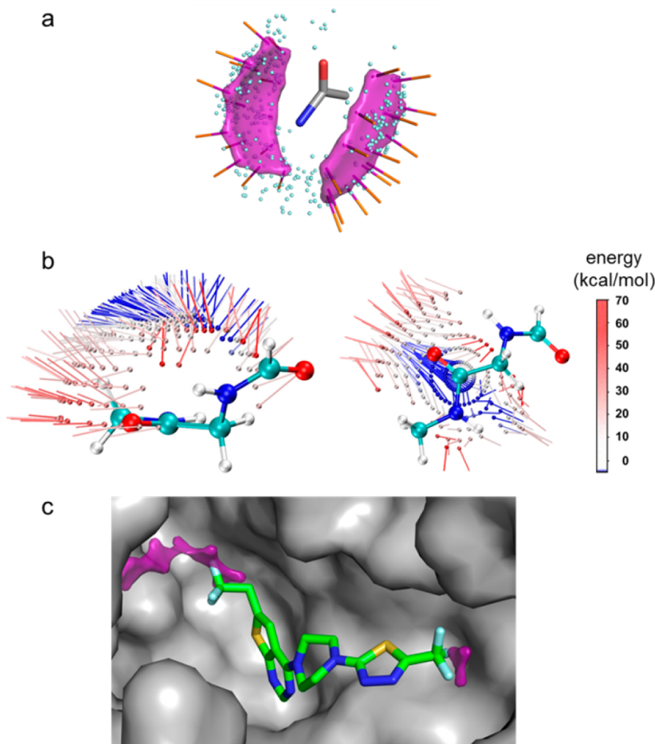
Figure 2. Prediction of favorable C–F...C=O interactions using FMAP algorithm. (a) Combined analysis of protein–ligand structures from PDB, with FMAP predictions of the potential fluorine positions and their representative C–F bonds relative to backbone peptide bond. Positions of fluorine atoms derived from the protein–ligand complexes found in PDB are shown as cyan points. FMAP prediction is shown as purple surface with orange vectors shown for representative C–F bonds. (b) Binding energy calculations (kcal/mol) for interaction of fluoromethane with a model peptide using MP2/6-31G(d) theory level as a function of C–F bond orientation. Distance between fluorine and carbonyl carbon is set to 3 Å. Fluorines are represented as small balls, and the C–F bonds are represented as sticks. Model peptide is presented in balls and sticks representation (carbon in cyan, oxygen in red, and nitrogen in blue). (c) FMAP prediction for the menin–MI-2-3 complex. Purple surface represents favorable positions for fluorine atoms to interact with protein backbone.
