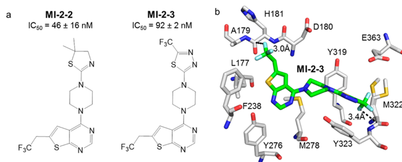
Figure 1. Inhibitors of the menin–MLL interaction containing CF 3 groups. (a) Structures and activities of MI-2-2 and MI-2-3. (b) Crystal structure of MI-2-3 bound to menin. Short C–F...C=O distances are shown using dashed lines.
