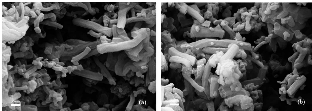
Fig. 3 SEM images of MCM-41 (a) and Ti-MCM-41 (b).
