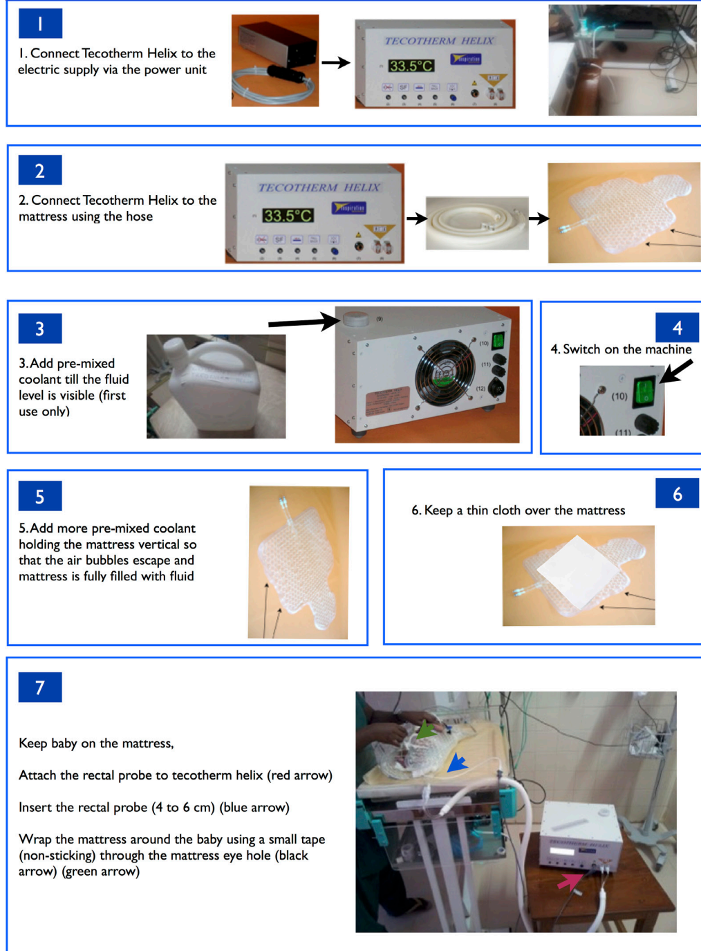
Figure 1 Setting up of Tecotherm HELIX cooling device.
