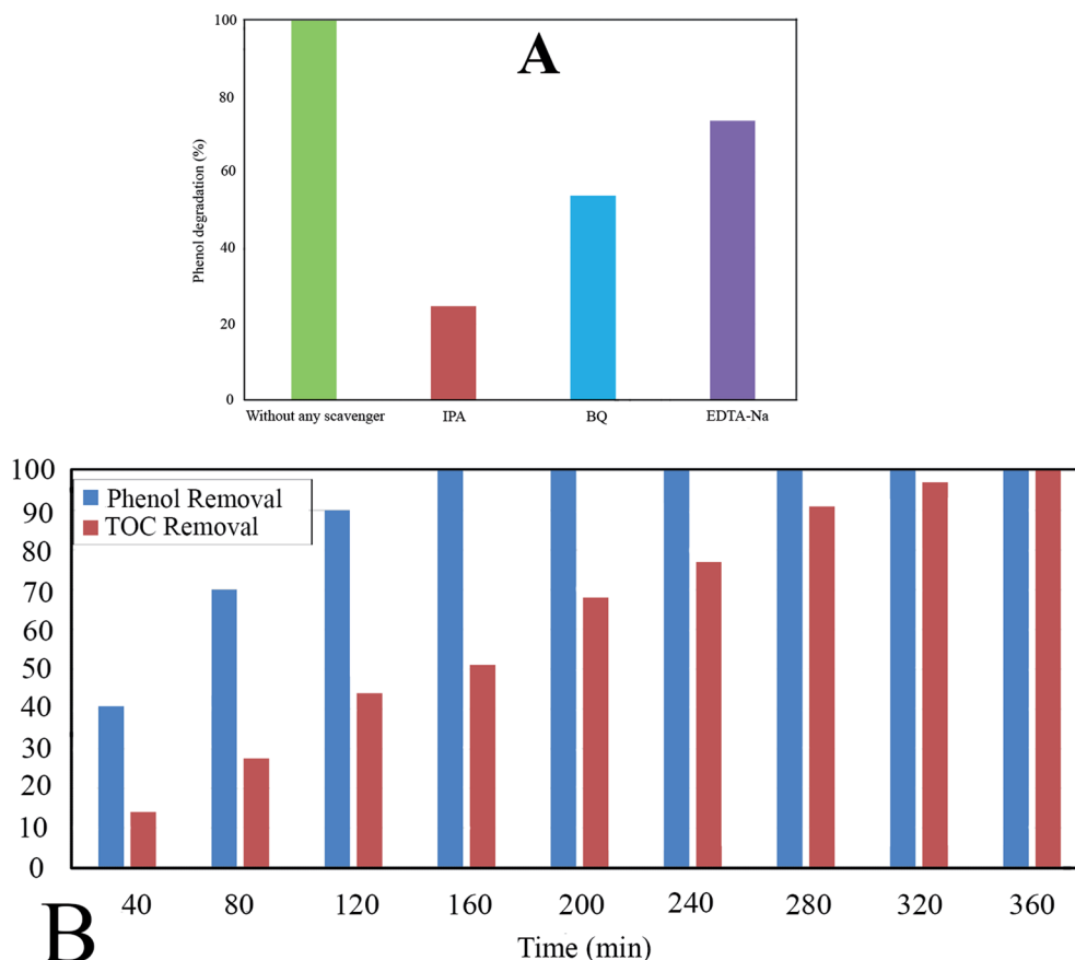
Fig. 10 (A) Ph-degradation efficiency in the presence of different radical scavengers (IPA, BQ, Na 2 -EDTA); (B) comparison of phenol removal and TOC removal at pH: 4, catalyst dosage: 0.6 \text{ g L}^{-1} , and phenol concentration: 60 ppm.
