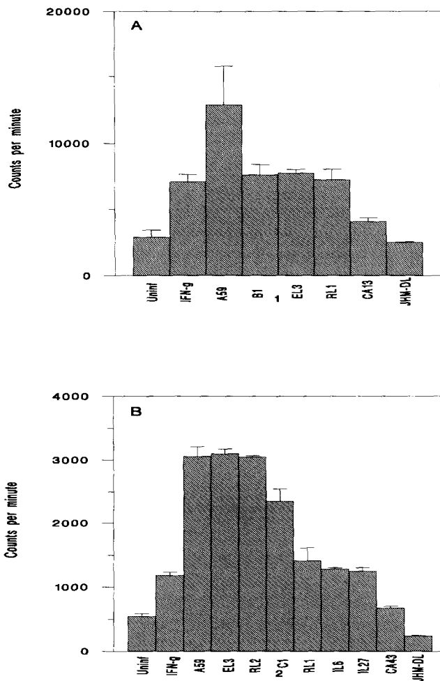
Figure 3. MHC class I ( K^b ) induction in primary astrocytes infected by A59 and recombinant A59/JHMV coronavirus strains. Data represent mean \pm SD of triplicate determinations. Data are also included for uninfected astrocytes exposed to IFN- \gamma (100 U/ml) for 48 h before assay on day 3 p.i. A and B are two experiments that are representative of four experiments yielding similar results.
