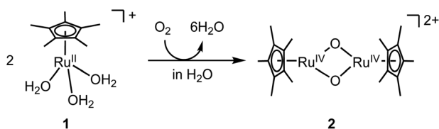
Fig. 1 Synthesis of bis( \mu -oxido) \text{Ru}_2^{\text{IV}} complex 2 from oxygenation of mononuclear \text{Ru}^{\text{II}} triaqua complex 1 in \text{H}_2\text{O} .
