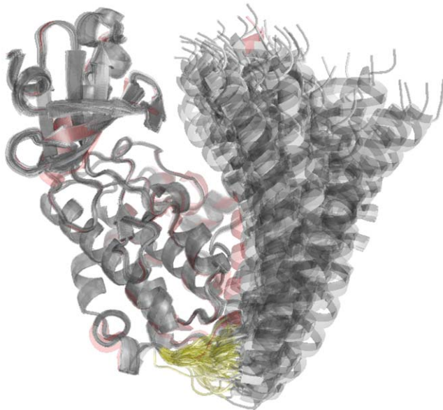
Figure 1. Opening of a CaMKII subunit. Overlay of 100 model structures created with MODELLER, where structural information was omitted for the four residues linking the kinase domain of CaMKII with the inhibitory helix. These four residues are shown in yellow. The structure corresponding to the published structure of the kinase domain (with the linker region intact, PDB ID: 2BDW, chain A) [13] is shown in red.
