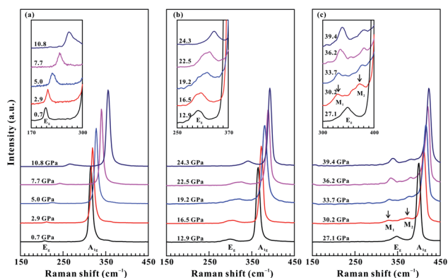
Fig. 2 Raman scattering spectra of SnS 2 at different pressure points up to 39.4 GPa in the process of compression under non-hydrostatic condition. (a) 0.7–10.8 GPa; (b) 12.9–24.3 GPa; (c) 27.1–39.4 GPa. Inset: the corresponding enlarged figures of the E g , M 1 and M 2 modes during compression.
