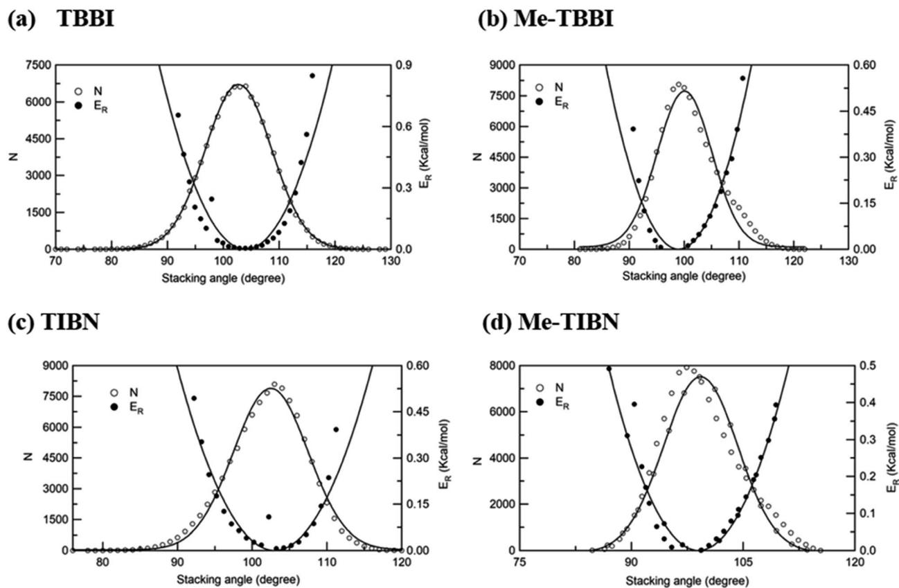
Fig. 2 Number of occurrence ( N ), relative energy ( E_R ) with respect to stacking angle for (a) TBBI, (b) Me-TBBI, (c) TIBN and (d) Me-TIBN molecules.
