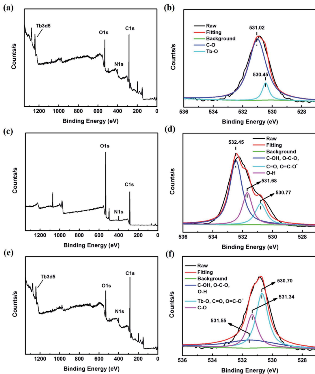
Fig. 3 (a) XPS of \text{Tb}(\text{acac})_2\text{phen} ; (b) high-resolution O 1s peak of \text{Tb}(\text{acac})_2\text{phen} ; (c) XPS ofhya; (d) high-resolution O 1s peak ofhya; (e) XPS ofTHNE; (f) high-resolution O 1s peak ofTHNE.
