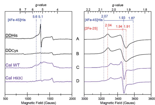
Fig. 4 X-band EPR spectra of distal domain and Cal, with low-field region on left; high-field region, on right. (A) DDHis ( 230 \mu M ) (B) DDCys ( 230 \mu M ) (C), Cal WT ( 200 \mu M ) (D) Cal H93C ( 200 \mu M ). All samples were prepared under identical conditions and reduced with dithionite in pH 8.8 buffer. Signal assignments for the [4Fe-4S]His and [2Fe-2S] clusters are indicated. Measurement conditions: microwave frequency 9.39 \text{ GHz} ; modulation frequency, 100 \text{ kHz} ; modulation amplitude, 10 \text{ Gauss} ; microwave power, 1 \text{ mW} (A and B), 10 \text{ mW} ( 500\text{--}2000 \text{ Gauss} C and D), 1 \text{ mW} ( 3000\text{--}4000 \text{ Gauss} C and D); sample temperature: 10 \text{ K} .
