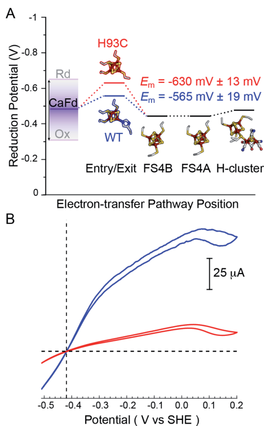
Fig. 3 (A) Thermodynamic landscape for electron transfer between the catalytic H-cluster in Cal and its redox partner ferredoxin. The scheme shows E_m values for the distal [4Fe-4S] cluster of WT Cal (blue) and H93C Cal (red) obtained in this study, in relation to the E_m range for reduced (Rd) and oxidized (Ox) CaFd, 21 the E_m 's of F-cluster relay comprised of [4Fe-4S] clusters FS4B and FS4A, and the formal potential of the H-cluster at pH 8.8. 19 (B) Electrocatalytic profiles of Cal WT (blue) and Cal H93C (red). Voltammograms were collected under 1 atm of H_2 at a potential scan rate of 1 \text{ mV s}^{-1} . Other experimental conditions are pH 7.0, 25^\circ \text{C} and an electrode rotation rate of 3500 rpm. The dotted horizontal line shows zero current.
