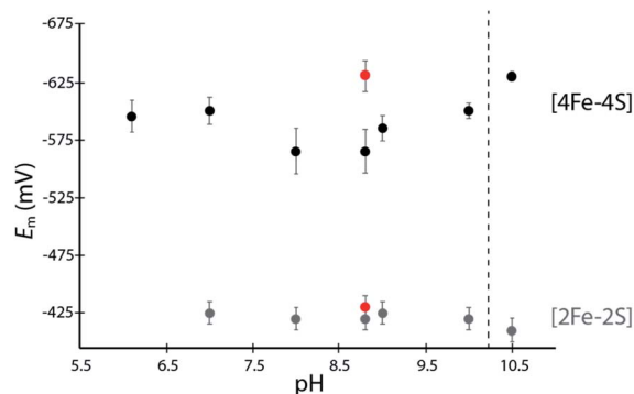
Fig. 2 Scatter plot of measured E_{\text{m}} values for DDHis (black dots) and DDCys (red dots) iron–sulfur clusters at various solution pH values. Error bars represent standard deviation from at least 5 scans.
