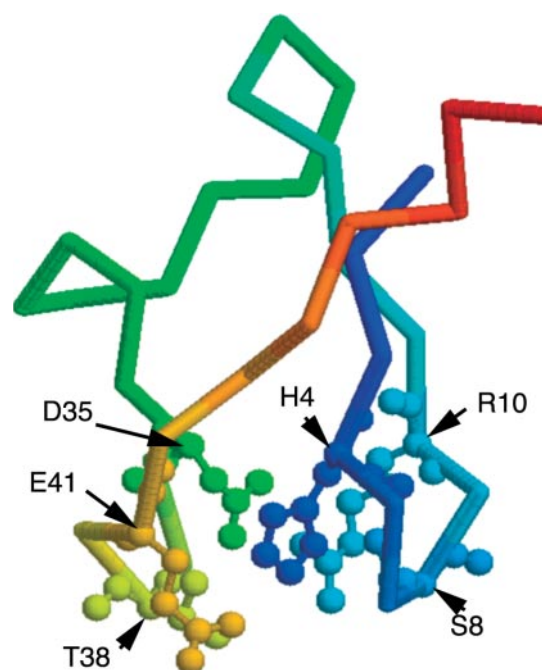
Figure 4. A RasMol rendition of the bovine ADK_lid structure. Residues 4, 8, 35 and 38 are mutated to cysteines in Gram-positive bacterial ADK_lid domains. Residues 10 and 41 are implicated in a structural capacity in variants lacking the cysteines, due to strong positive relationships between their identities, and those of the 4, 8, 35, 38 quadruple.
