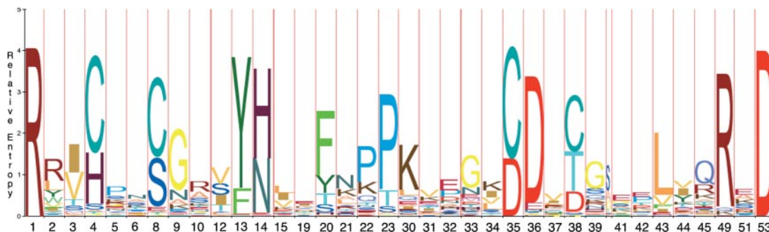
Figure 3. A LogoMat-M HMM-Logo visualizing the HMM defined by the Pfam ADK_lid training sequence set, renumbered to match the complete 299-member predicted family. The logo provides a convenient visualization of the identity probabilities at each position, and to what extent each position contributes to the information content of the model, but it does not suggest the apparent requirement for either of the alternate C4, C8, C35, C38 or H4, H8, R10, D35, T38, E41 motifs that are found in the actual sequences.
