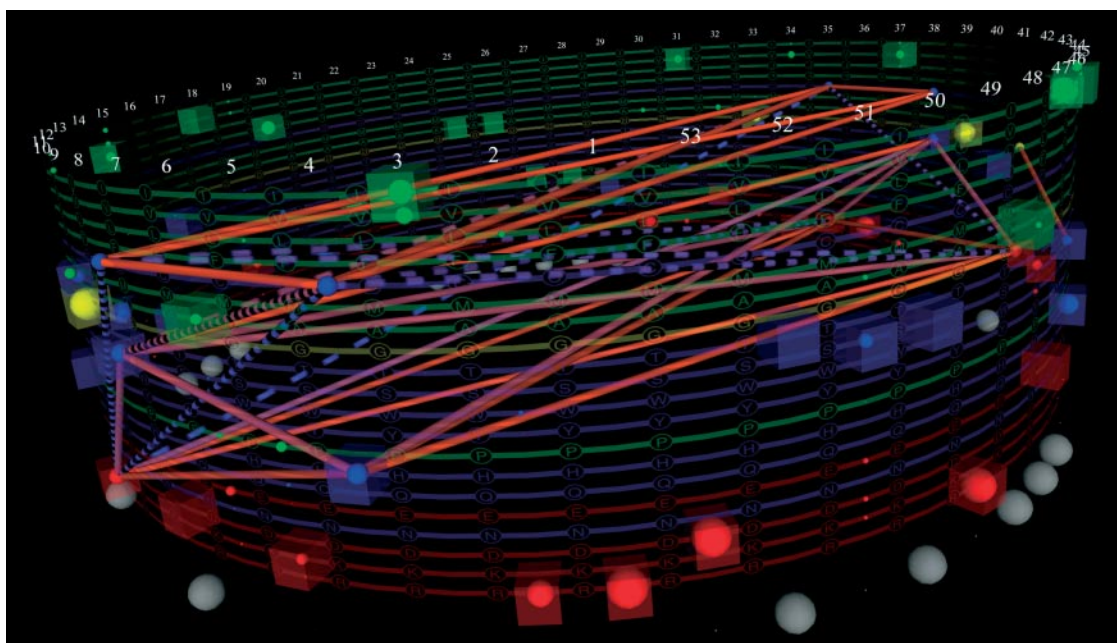
Figure 2. A StickWRLD diagram showing related positions in the ADK_lid domain. The positively related cysteines at 4, 8, 35 and 38 stabilize the domain structure using bound zinc in a conformation analogous to a zinc finger, while the positively related histidine, serine, aspartic acid and threonine in the same positions stabilize the same domain structure using a network of hydrogen bonds. The amino acid identities are arranged vertically by their Kyte–Doolittle hydropathy score, and are colored using Branden and Tooze's classical coloring and grouping of residues by hydrophobic character. Consensus identities in each position are highlighted by a transparent unit cube. In a live VRML browser, this diagram is completely navigable and the viewer can rotate, move and zoom the 3D diagram to examine details of any portion.
