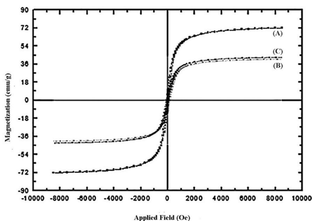
Figure 5. Magnetization hysteresis loop of (A); \text{Fe}_3\text{O}_4 ; (B); \text{Fe}_3\text{O}_4/\text{SA}/\beta\text{-CD} and (C); \text{Fe}_3\text{O}_4/\text{SA}/\beta\text{-CD}/\text{CP} respectively.
