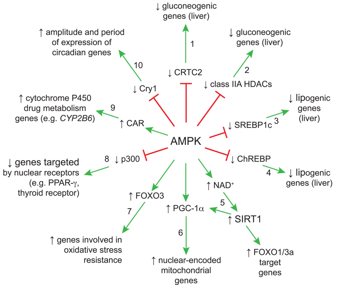
Figure 3. Effects of AMPK activation on transcription. Upward/downward arrows indicate that the target transcription factor or co-activator (inner wheel) or target genes (outer wheel) are activated/inactivated. Note that SIRT1 (on spoke 5) deacetylates both FOXO family transcription factors and the transcriptional co-activator PGC-1 \alpha .
