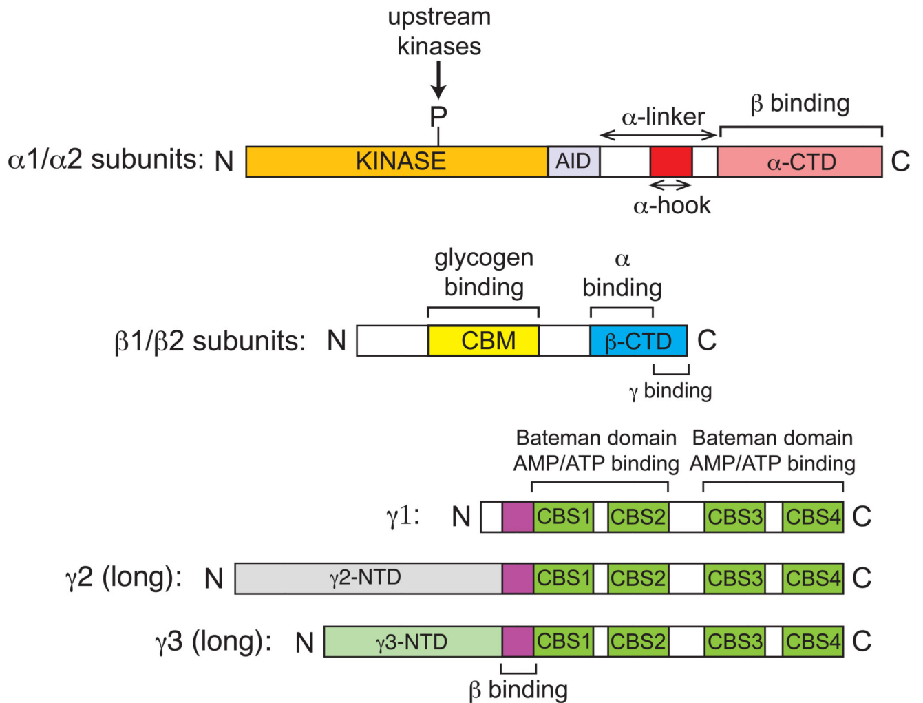
Figure 1. Domain structure of the \alpha , \beta and \gamma subunits of AMPK and their isoforms. KEY: \alpha -subunits: AID, auto-inhibitory domain, \alpha -CTD, C-terminal domain; \beta -subunits: CBM, carbohydrate-binding module; \beta -CTD, C-terminal domain; \gamma subunits: CBS1, CBS2, CBS3, CBS4, cystathione \beta -synthase repeats; \gamma 2-NTD, N-terminal extension of “long” version of \gamma 2 subunit; \gamma 3-NTD, N-terminal extension of “long” version of \gamma 3 subunit.
