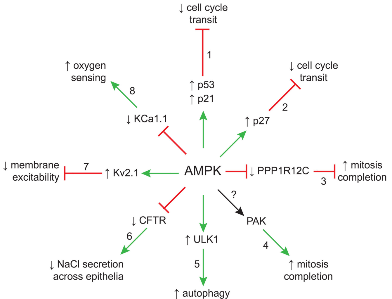
Figure 4. Effects of AMPK activation other than on metabolism and/or transcription. Upward/downward arrows indicate that the functions of the target protein (inner wheel) or target process (outer wheel) are activated/inactivated.
