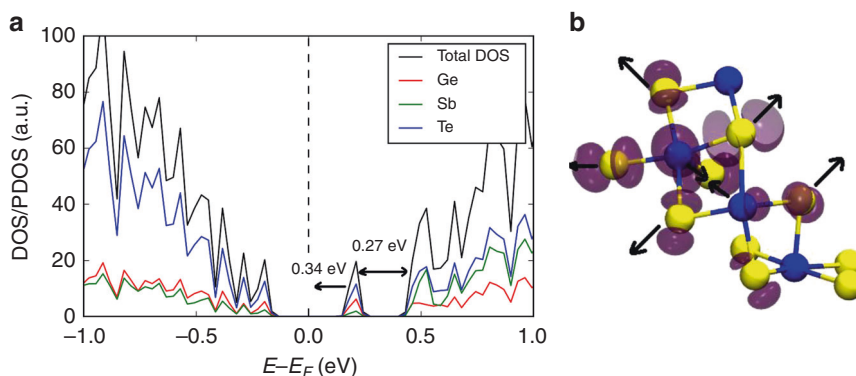
Fig. 7 The mid-gap defect states as deep electron traps. a Total and partial electronic densities of states (DOS/PDOS) of an amorphous 225GST model (glass sample #14 from Supplementary Table 1) with a mid-gap defect state located at 0.27 eV below the bottom of the conduction band. An extra electron can occupy the mid-gap electronic state, and this state shifts by 0.34 eV towards the valence-band maximum following geometry relaxation, as indicated by the arrow. The mid-gap localised defects in the amorphous 225GST models are able to capture electrons and correspond to deep traps in the band gap of the material. b Spin-density distribution and atomic geometry of an electron trap in the glass model #14 from Supplementary Table 1, which has a mid-gap electronic state. The extra electron is well localised on a small cluster of Ge atoms within the glass structure. Five-coordinated Ge atoms are associated with the electron localisation and the structural motif of the electron defect centre has a crystalline-like character, which characterises the mid-gap defect states identified in the amorphous models. Arrows indicate the direction of atomic displacements following electron trapping. Ge atoms are blue and Te atoms are yellow. The isovalue of the spin density (light-purple isosurface) is equal to 0.001
