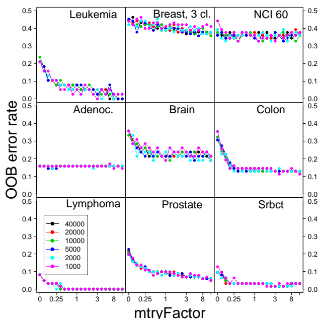
Figure 1 Out-of-Bag (OOB) vs mtryFactor for the nine microarray data sets. mtryFactor is the multiplicative factor of the default mtry ( \sqrt{\text{number} \cdot \text{of} \cdot \text{genes}} ); thus, an mtryFactor of 3 means the number of genes tried at each split is 3^2 \cdot \sqrt{\text{number} \cdot \text{of} \cdot \text{genes}} ; an mtryFactor = 0 means the number of genes tried was 1; the mtryFactors examined were = {0, 0.05, 0.1, 0.17, 0.25, 0.33, 0.5, 0.75, 0.8, 1, 1.15, 1.33, 1.5, 2, 3, 4, 5, 6, 8, 10, 13}. Results shown for six different ntree = {1000, 2000, 5000, 10000, 20000, 40000}, nodesize = 1.
