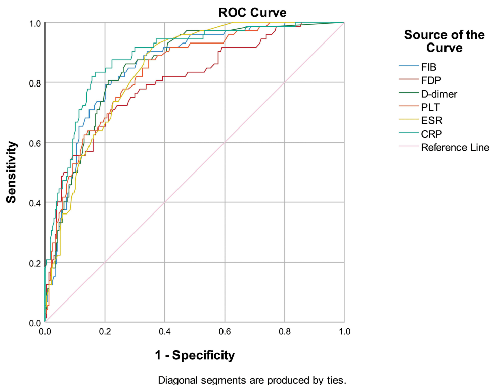
Figure 1 Receiver operating characteristic curves of FIB, FDP, D-dimer and inflammatory indexes in differentiating severe from non-severe UC patients.
