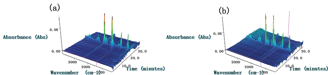
Fig. 9 3D-IR spectra of the gas products of NC (a) and \text{Cr}_2\text{O}_3/\text{NC} (b) at the heating rate of 10 °C min -1 .
