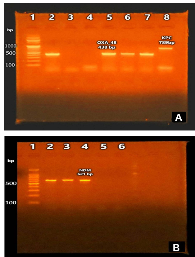
Figure 2 PCR results for carbapenemase genes. (A) Agarose gel electrophoresis of bla KPC and bla OXA-48 amplicons. Lane (1): DNA ladder 100 bp, lanes (2, 5, 6, 7): positive for bla OXA-48 gene (438bp), lane (8): positive for bla KPC gene (789bp). (B) Agarose gel electrophoresis of bla NDM amplicons. Lane (1): DNA ladder 100 bp, lanes (2–4): positive for bla NDM gene (621bp).
