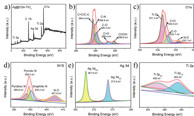
Fig. 3 XPS spectra of Ag@CDs- \text{TiO}_2 hybrid NFs: (a) full-range, (b) C 1s, (c) O 1s, (d) N 1s, (e) Ag 3d, (f) Ti 2p.
