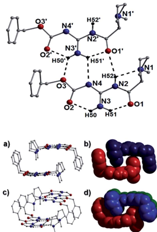
Fig. 10 (Top): Intermolecular H-bonding arrangement (dashed lines) between two crystallographically equivalent 25a units. Selected distances: O3' \cdots (H50')N3' = 2.20 \text{ \AA} ; N4' \cdots (H51')N3' = 2.63 \text{ \AA} and N2(H52) \cdots O1' = 2.58 \text{ \AA} . Note: intramolecular H-bonding also shown (dashed lines). (Bottom): Regular (a and c) and space-fill (b and d) views of the packing arrangement observed in 25a . Each unit (in b and d) is represented by a different colour to highlight the space efficient interdigitation of the U-shaped organic units in 25a .
