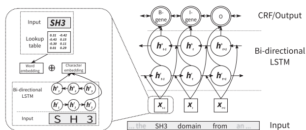
Fig. 1. CRF-LSTM architecture. For instance, for the word w_{t-1} = \text{'SH3'} from the input sentence S , the character-based representation is computed by applying a bi-directional LSTM onto the sequence of its characters 'S', 'H', '3'. The resulting embedding is concatenated with the corresponding word embedding, trained on a huge corpus. This word representation is then processed by another bi-directional LSTM and finally by a CRF layer. The output is the most probable tag sequence, as estimated by the CRF
