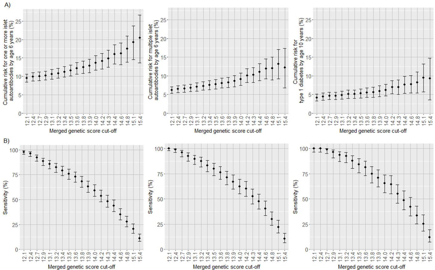
Fig 5. Cumulative risks and the proportion of cases identified for 1 or more islet autoantibodies, multiple islet autoantibodies, and type 1 diabetes in TEDDY children with the HLA DR3/DR4-DQ8 or DR4-DQ8/DR4-DQ8 genotype according to increasing thresholds of the merged genetic score. Cumulative risk for developing islet autoantibodies by age 6 years and diabetes by age 10 years (A) and the proportion of cases positive for islet autoantibodies by age 6 years and diabetes by age 10 years (sensitivity; B) in TEDDY children with the HLA DR3/DR4-DQ8 or DR4-DQ8/DR4-DQ8 genotype stratified by their merged genetic score. The risk and sensitivity are shown for each increment in the genetic score by the 5th percentile of scores in the TEDDY children, ranging from >12.1 (the 5th percentile of children) to >15.4 (the 95th percentile of children). The risk and sensitivity are shown for the development of 1 or more islet autoantibodies (left panels), multiple islet autoantibodies (middle panels), and type 1 diabetes (right panels). Error bars indicate 95% confidence intervals.
