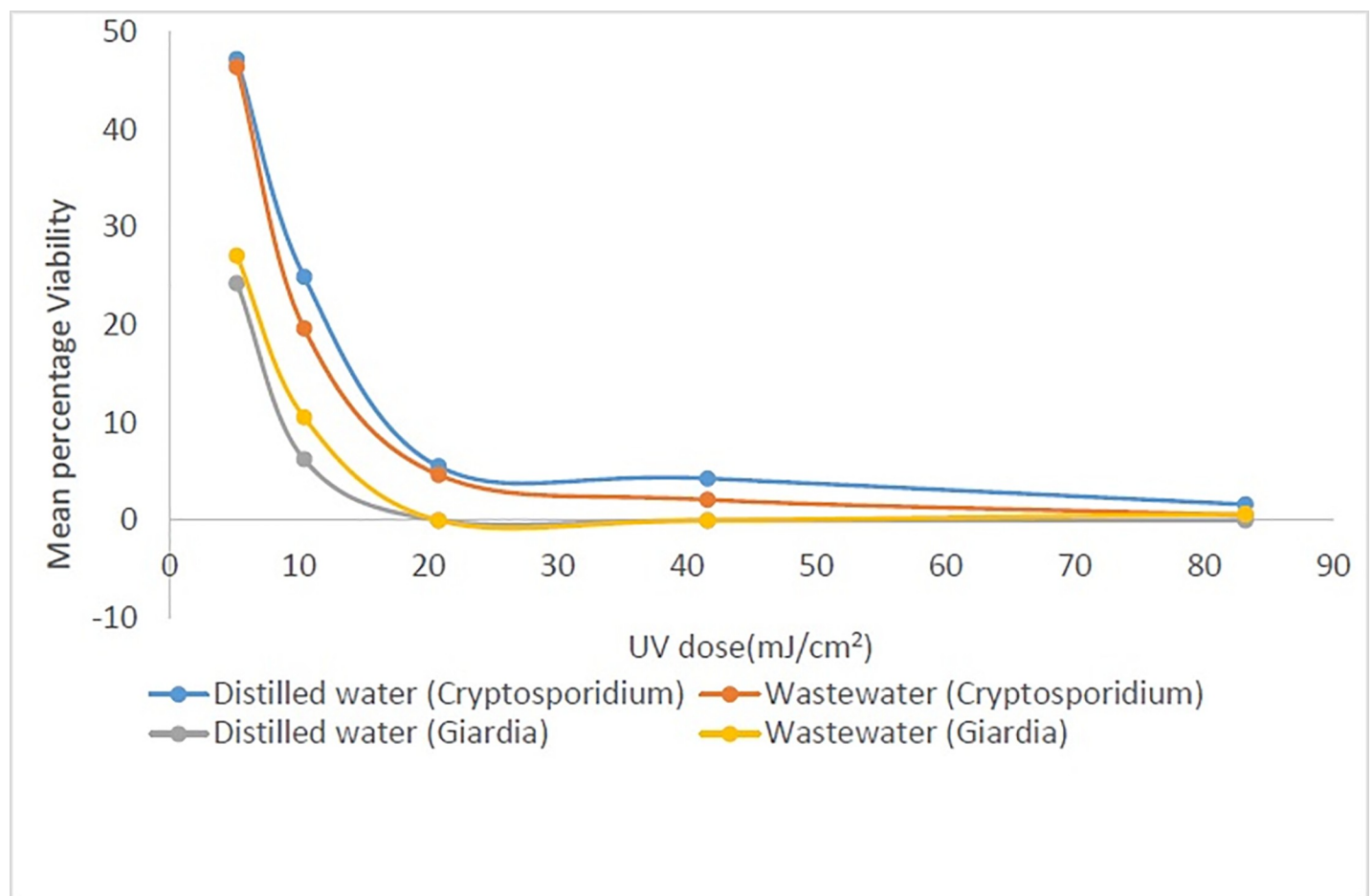
Fig 1. Mean percentage viability of Cryptosporidium and Giardia related to UV doses in treatment with spiked samples in distilled water and wastewater samples.
