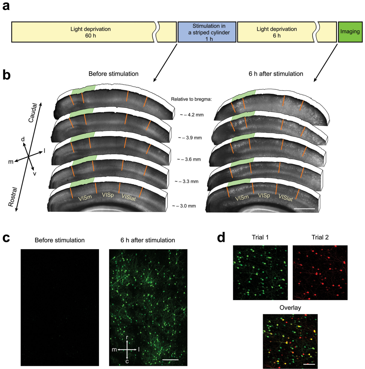
Figure 1. Arc::dVenus expression pattern in the visual cortex following structured light stimulation. (a) Visual stimulation paradigm. Prior to stimulation mice were single-housed in their home cages in the dark for 60 hours. After light deprivation period mice were placed into illuminated cylinder with vertical black and white stripes for 1 hour and then transferred back into dark home cage for 6 hours until imaging. (b) Postmortem IHC analysis of Arc::dVenus expression in mouse visual cortex. Visual area borders are based on Allen Mouse Brain Reference Atlas ( http://mouse.brain-map.org ). Left panel: virtually no Arc::dVenus is present in the visual cortex at the end of 60-hour light deprivation period. Right panel: 6 hours after visual stimulation Arc::dVenus is present largely in the medial
