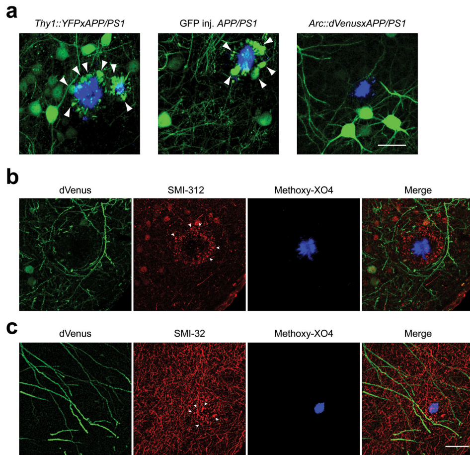
Figure 4. Neurons with dystrophic neurites do not express Arc::dVenus in response to a stimulus. (a) Maximum intensity projections of in vivo image stack of Thy1::YFPxAPP/PS1 transgenic mouse, APP/PS1 mouse injected with GFP AAV2 virus and Arc::dVenusxAPP/PS1 mouse 6 hours after visual stimulation. Blue—amyloid plaques visualized with methoxy-XO4; green—YFP, GFP or dVenus fluorescence. Arrowheads point at YFP- and GFP-filled neuritic dystrophies characteristic for the APP/PS1 model. Scale bar = 30 μm. (b,c) Postmortem immunostaining of Arc::dVenusxAPP/PS1 mouse brain tissue acquired 6 hours after visual stimulation for Arc::dVenus (with anti-GFP antibody, green channel) showed no co-localization of experience-dependent dVenus expression with either axonal (SMI-312, (b) ) or dendritic (SMI-32, (c) ) neurofilament staining (red channel) that typically accumulates in dystrophic axons or dendrites (arrowheads) around amyloid plaques (methoxy-XO4, blue channel). Scale bar = 30 μm is shared by (b,c) .
