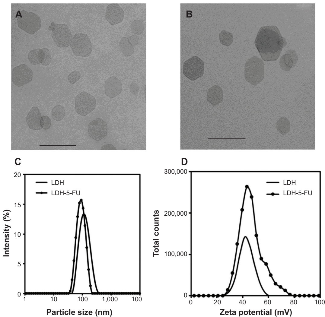
Figure 1 Featured structure of LDH and LDH-5-FU nanohybrids. Notes: (A–B) Transmission electron microscopy images of LDH and LDH-5-FU. The scale bar represents 200 nm. (C) Particle size distribution of LDH and LDH-5-FU from dynamic light scattering. (D) Zeta potential of LDH and LDH-5-FU. Abbreviations: LDH, layered double hydroxide; 5-FU, fluorouracil.
