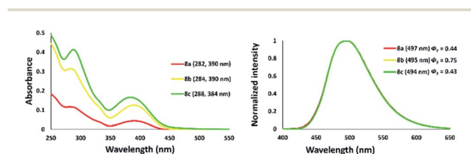
Fig. 13 Absorption (right) and emission spectra of zinc–thiazole complexes 8a–c in THF [ 10^{-5} M].
