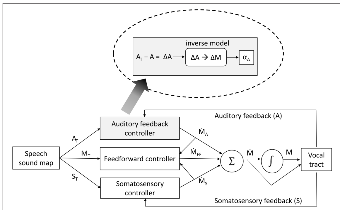
Figure 1: Schematic of the DIVA model (adapted from Guenther, 2016). The inset shows the calculations within the auditory feedback controller. A_T = Auditory Target; M_T = Motor Target; S_T = Somatosensory Target; \dot{M}_A and \dot{M}_S = corrective movement commands from auditory and sensory routes, respectively; \dot{M}_{FF} = feedforward movement command; \dot{M} = overall movement command. M = motor position command; \alpha_A = gain factor.
