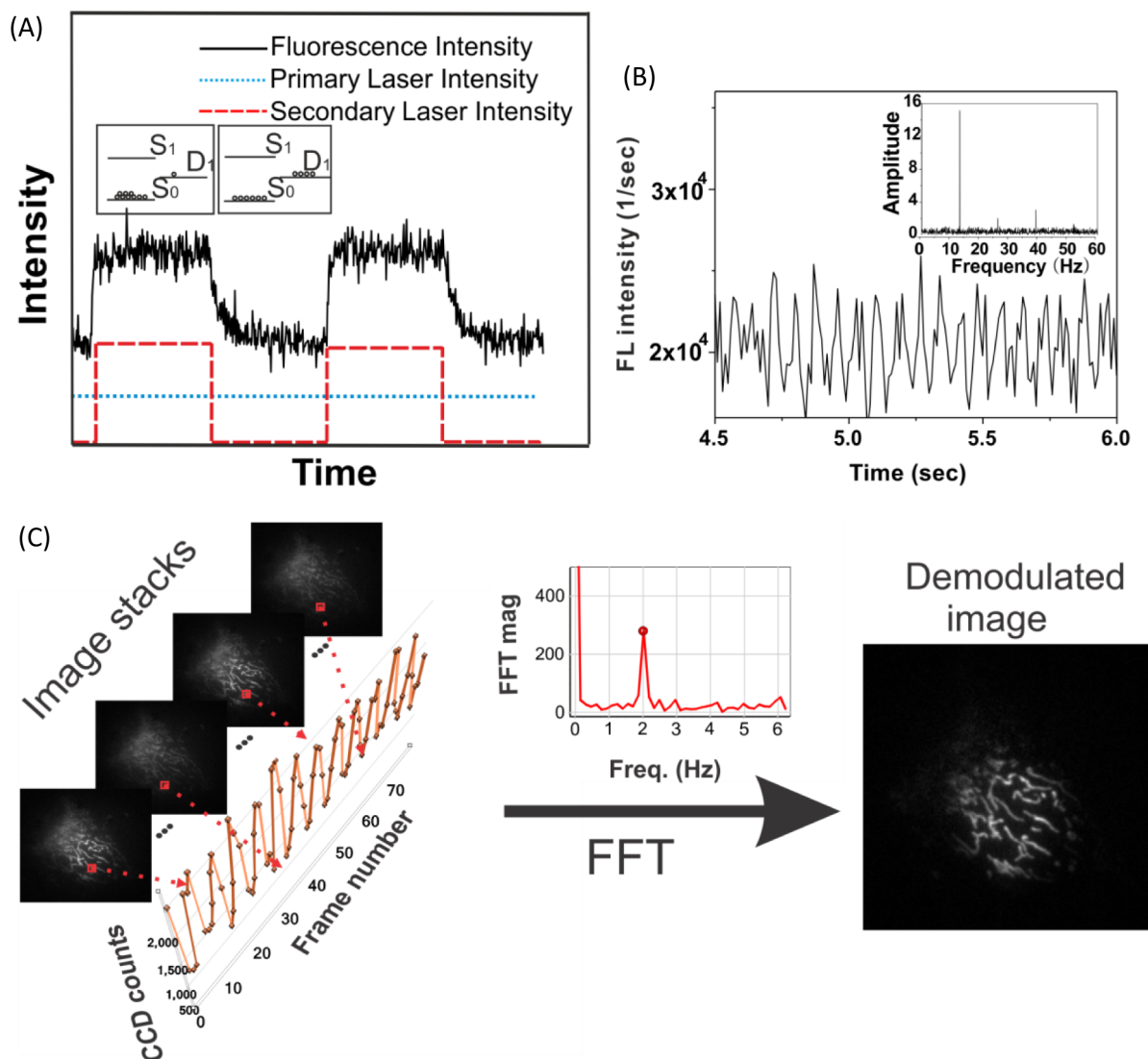
Figure 3. (A) Fluorescence response of an optically modulated blue fluorescent protein (modBFP/H148K) with constant primary excitation and modulated secondary excitation. The insets show Jablonski diagrams representing dark/bright populations. (B) Time trace of aqueous modBFP/H148K with 372 nm primary excitation and 514 nm secondary excitation modulated at 13 Hz. The inset shows the fast Fourier transform (FFT) of the bulk intensity trajectory, recovering the modulation frequency encoded in the fluorescence signal. (C) Analysis of optically modulated image stacks acquired with SAFIRE by taking the Fourier transform of each pixel's intensity trajectory. The demodulated image is formed from the FFT amplitude at each pixel.
