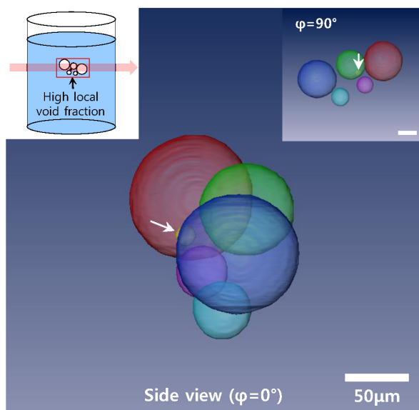
Figure 3 | Geometric analysis of rising microbubbles. Side view of a reconstructed bubble cluster with six microbubbles. The sizes and 3-D positions of six bubbles are clearly identified despite substantial horizontal overlaps between the bubbles, as illustrated in the inset on left-top corner. (Inset on right-top corner: side view at \varphi = 90^\circ , scanning time for 60 projections: 1.0 s, effective pixel size: 1.0 \mu\text{m} ).
