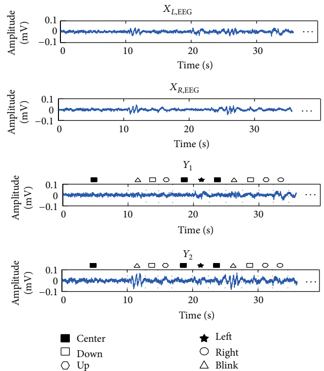
FIGURE 3: Example of raw EEG signals X_{L,\text{EEG}} and X_{R,\text{EEG}} , from the left and right electrodes, respectively, and processed signals Y_1 and Y_2 . The symbols represent blink and eye movement classes.
