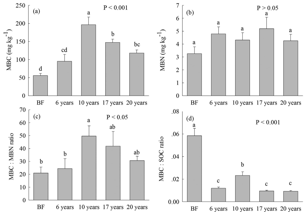
Figure 1. (a) Soil microbial biomass carbon (MBC), (b) Soil microbial biomass nitrogen (MBN), (c) MBC:MBN ratio and (d) MBC:SOC ratio (mean \pm SE, n = 9 ) in bare flat (BF) and different invasion times (6, 10, 17 and 20 years) of S. alterniflora soils (0–30 cm depth). Different lower case letters over the bars indicate statistically significant differences at \alpha = 0.05 level across the S. alterniflora invasion chronosequence.
