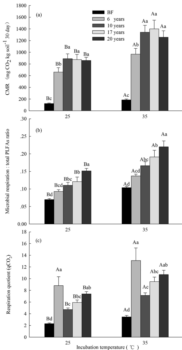
Figure 4. (a) Cumulative microbial respiration (CMR), (b) Microbial respiration on a per-unit-PLFAs basis and (c) Respiration quotient ( q\text{CO}_2 ) after 30-days incubation under different temperature treatments (25°C and 35°C) (mean \pm SE, n = 9 ) in bare flat (BF) and different invasion times (6, 10, 17 and 20 years) of S. alterniflora soils (0–30 cm depth). Different lower case letters over the bars indicate statistically significant differences at \alpha = 0.05 level across the S. alterniflora invasion chronosequence. Different upper case letters over the bars indicate statistically significant differences at \alpha = 0.05 level between incubation temperature.
