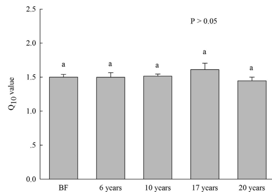
Figure 5. Temperature sensitivity (Q 10 ) of microbial respiration after 30-days incubation time at 25 °C and 35 °C (mean ± SE, n = 9) in bare flat (BF) and different invasion times (6, 10, 17 and 20 years) of S. alterniflora soils (0–30 cm depth). Different lower case letters over the bars indicate statistically significant differences at \alpha = 0.05 level across the S. alterniflora invasion chronosequence.
