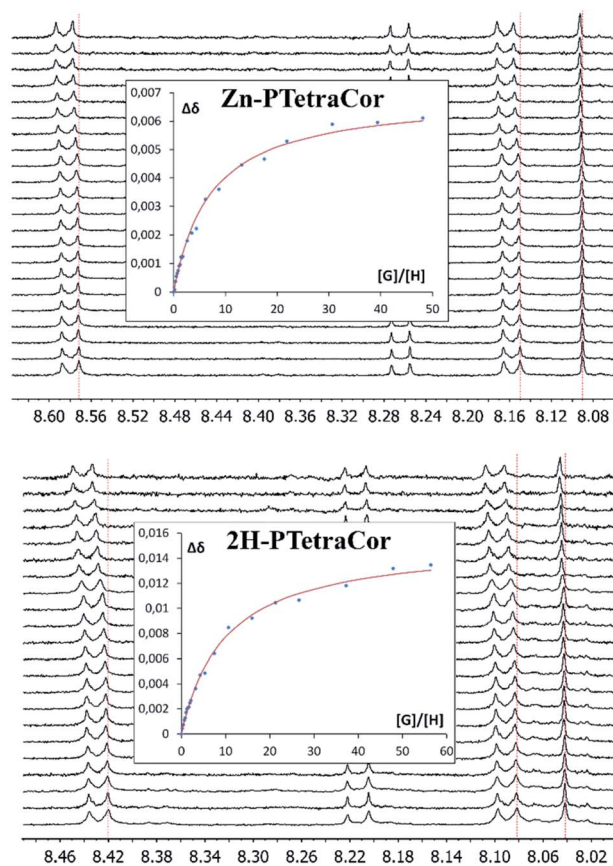
Fig. 3 ^1\text{H} NMR spectra (500 MHz, toluene- d_8 ) showing the H_6 , H_7 , and H_{10} chemical shifts (see ESI† for labelling scheme) of Zn-PTetraCor (top) and 2H-PTetraCor (bottom) upon the addition of aliquots of C_{60} . Insets: plots of the changes in chemical shift against [G]/[H] , where G (guest) is C_{60} and H (host) is Zn-PTetraCor or 2H-PTetraCor . The red line corresponds to the nonlinear fitting of \Delta\delta for H_6 to a 1 : 1 binding isotherm. [H] = 10^{-4} M. The titration was carried out by adding known portions of a stock solution of C_{60} or C_{70} ( [G] = 10^{-3} M). Note: the dotted red line over the spectrum is a guide for the eye.
