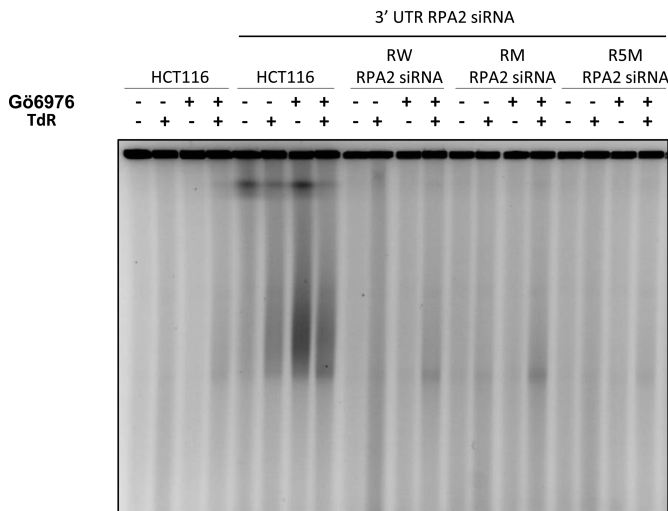
Figure 6. DSB analysis of HCT116 and strains expressing wild type and mutant RPA2. Parental HCT116 and strains ectopically expressing wild type or mutant RPA2 were depleted of endogenous RPA2 by transfection of the 3' UTR siRNA before a 24 h treatment with 1 \mu M Gö6976 and 2 mM thymidine. Cells were then harvested for analysis of DSBs by pulsed field gel electrophoresis. RPA2 depletion triggers DSB formation in HCT116 but this is rescued by ectopic expression of mutant or wild type RPA2. Neither thymidine nor CHK1 inhibitors alone or in combination enhance DSB formation in RPA2 depleted cells ectopic expression of mutant RPA2s is still able to rescue HCT116 from DSB formation.
