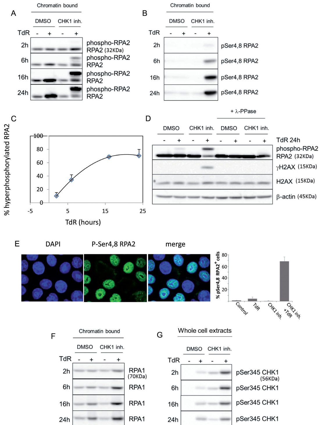
Figure 1. Nuclear RPA2 is extensively hyperphosphorylated in HCT116 cells treated with CHK1 inhibitor and thymidine. HCT116 cells treated or not treated with the CHK1 inhibitor G66976 in presence or absence of 2 mM thymidine were harvested at the indicated times and cytosolic, nuclear soluble or chromatin bound fractions were isolated. RPA2 (A) or pSer4,8-RPA2 (B) in the chromatin fractions were then analysed by western blotting. Densitometric measurements of phosphorylated RPA2 indicate that up to 70% of chromatin bound RPA2 is hyperphosphorylated (C). (D) Whole cell extracts obtained from cells treated with thymidine for 24 h in the presence or absence of the CHK1 inhibitor in the right lanes of this blot were treated with λ-phosphatase to confirm that the slower migrating band was the result of phosphorylation of RPA2. A blot of γH2AX is presented as a control to confirm the effectiveness of the phosphatase treatment. (E) Cultures of HCT116 cells treated for 24 h with G66976 in presence or absence of 2mM thymidine were fixed and stained for P-Ser4,8 RPA2 and the fraction of cells staining for this modified protein was determined by immunofluorescence. (F) Extracts prepared for panel A were also analysed for RPA1 content. (G) Whole cell extracts prepared from HCT116 cells treated as above were probed with an antibody for pSer345CHK1. Blots of all cellular fractions from this experiment are presented in Supplementary Figure S1. A western blot of those samples probed with an antibody for the origin binding protein ORC2 is also presented in this figure as a control for the cellular fractionation and gel loading.
