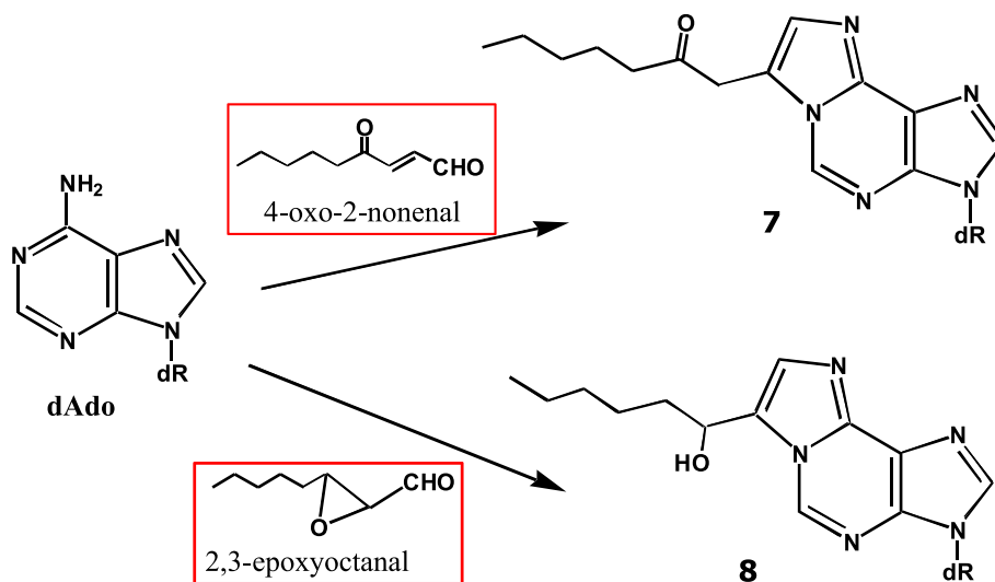
Fig. 12 Adduct formation of dAdo in an \omega -6-fat-hemin peroxidation model system. Mutagens involved in the adduct formation are shown in the red boxes
