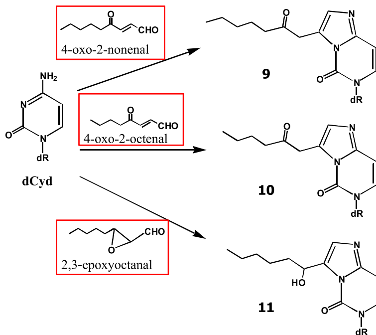
Fig. 13 Adduct formation of dCyd in an \omega -6-fat-hemin peroxidation model system. Mutagens involved in the adduct formation are shown in the red boxes
