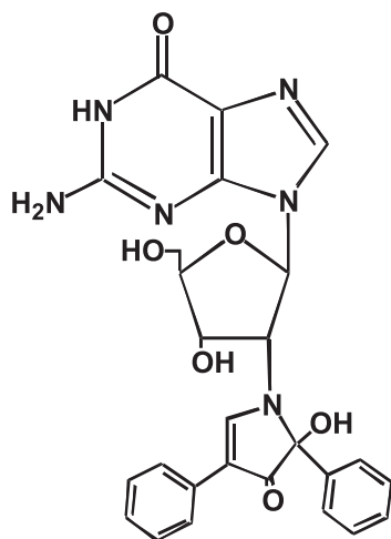
Fig. 4 Structure of the fluorescent guanosine derivative, FG
