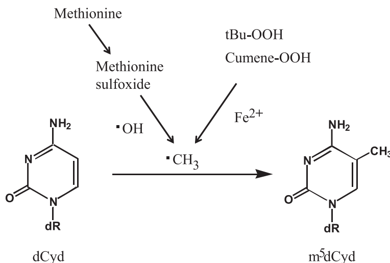
Fig. 14 Free radical-mediated dCyd C-5 methylation
