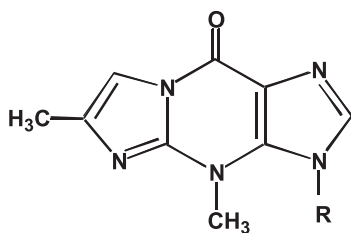
Fig. 1 Structure of wyosine
