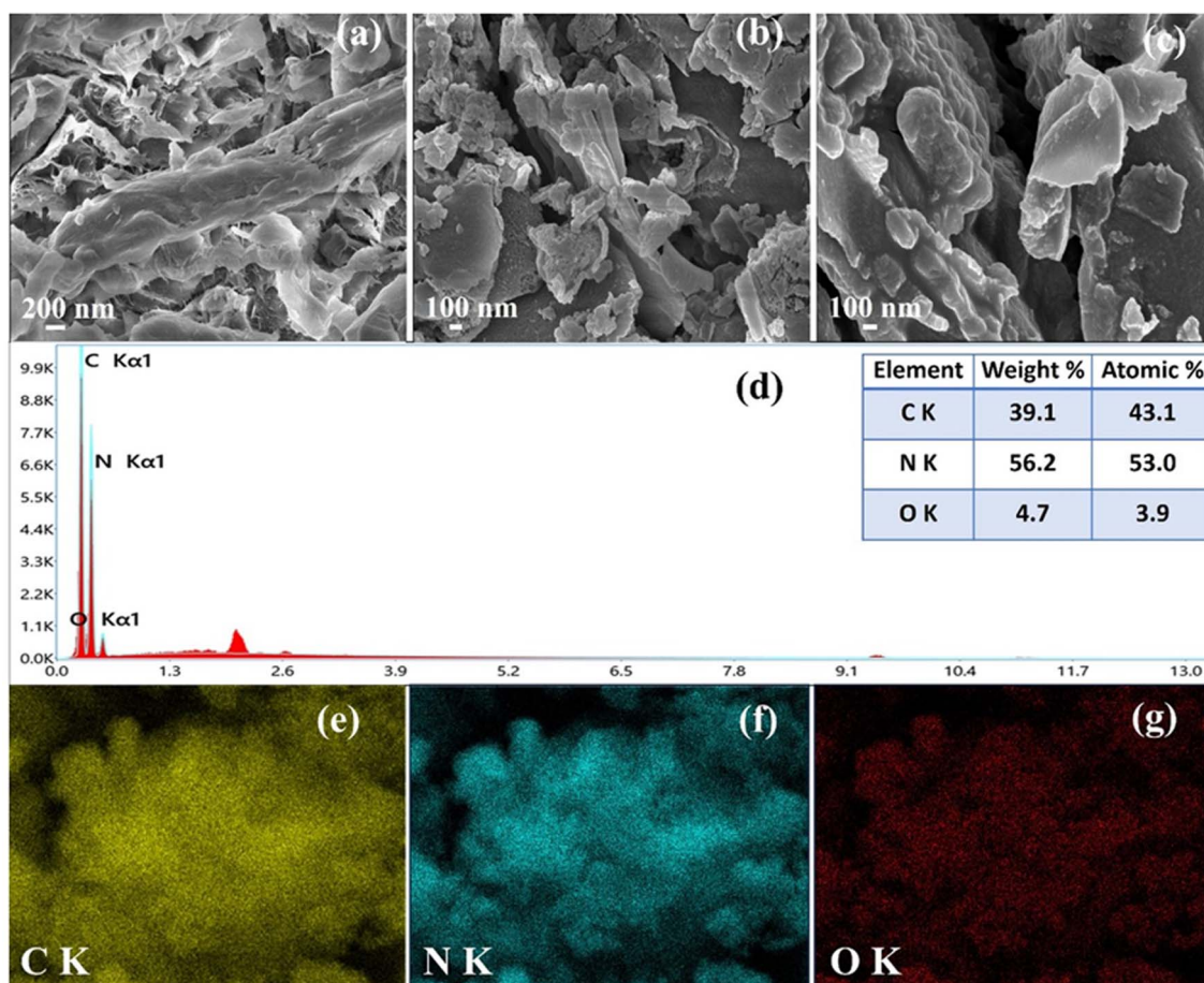
Fig. 6 SEM morphological analysis of (a) MBLC (b) g-C 3 N 4 (c) g-C 3 N 4 /C-MBLC (d) EDS of g-C 3 N 4 /C-MBLC and (e–g) elemental mapping of g-C 3 N 4 /C-MBLC (C, N and O).
