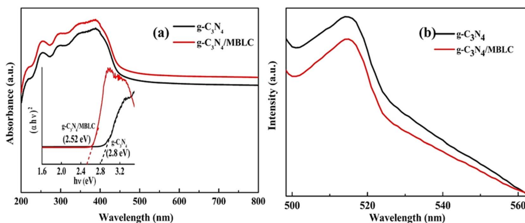
Fig. 7 (a) UV-vis-DRS, and (b) PL of the as-synthesized g-C 3 N 4 and g-C 3 N 4 /C-MBLC composite.
