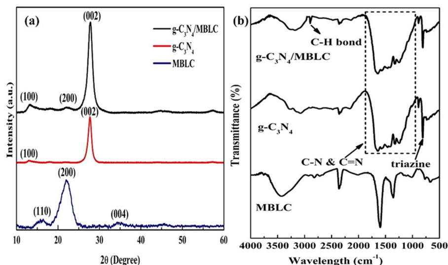
Fig. 2 (a) XRD pattern and (b) FTIR analysis of g-C 3 N 4 , MBLC, and g-C 3 N 4 /MBLC.
