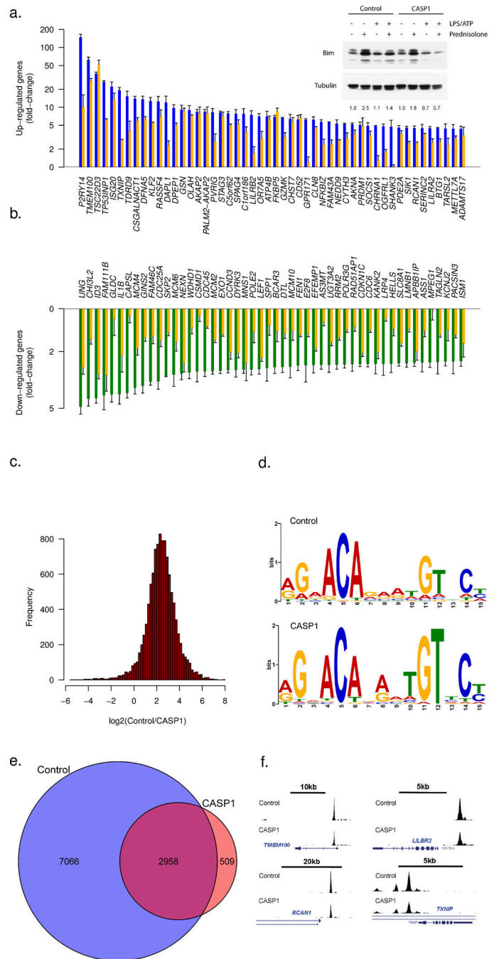
Figure 3. Transcriptional modulation induced by glucocorticoids is diminished by CASP1 Genome-wide gene expression was measured ( n = 4 ) with median values shown (panels A and B, error bars depict median absolute deviation) and fold-differences (with or without prednisolone treatment) were compared between control cells treated with prednisolone and the same cells not treated with prednisolone or in cells with enforced expression and activation of CASP1 treated with prednisolone or not. The top 50 genes activated (blue bars) and repressed (green bars) by prednisolone in untreated control cells are shown, with the fold-change in CASP1 overexpressing cells shown by the adjacent gold bars. Additionally,
