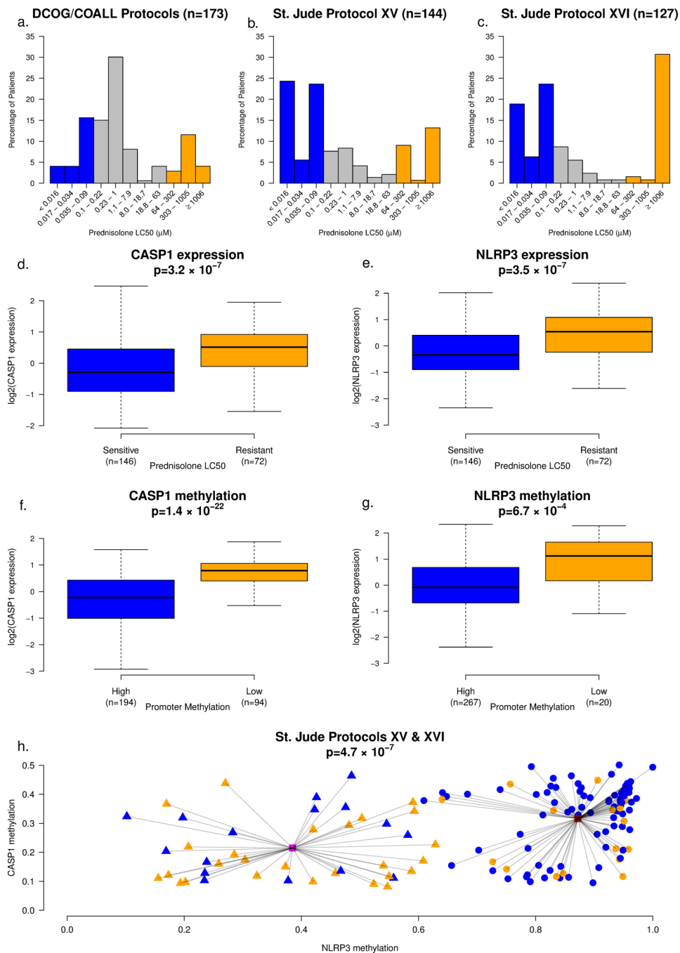
Figure 1. Glucocorticoid resistant leukemia cells have higher expression and hypo-methylation of CASP1 and NLRP3 genes
