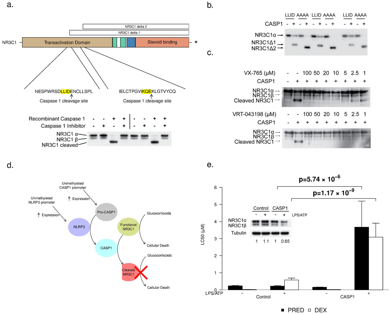
Figure 2. CASP1 cleaves the glucocorticoid receptor and increases resistance to glucocorticoids Bioinformatic analysis of the glucocorticoid receptor amino acid sequence (panel A, top) revealed a putative CASP1 cleavage site (LLID) in the glucocorticoid receptor (NR3C1) transactivation domain that is similar to a previously reported CASP1 cleavage site in the androgen receptor. Enzymatic assays revealed that recombinant CASP1 cleaves the glucocorticoid receptor and that this cleavage was inhibited by a CASP1 tetrapeptide inhibitor (panel A, bottom). Site directed mutagenesis of NR3C1 at the putative cleavage site (LLID motif) blocked CASP1 cleavage at this location and revealed a secondary CASP1 cleavage site more proximal to the carboxy terminus of the protein, as evidenced by a smaller enzymatic product (panel B). Further inhibition studies showed that small molecule inhibitors VX-765 and VRT-043198 (panel C) can also inhibit recombinant CASP1 cleavage of NR3C1, with VRT-043198 having higher inhibitory activity. Enforced expression of CASP1 in a human leukemia cell line (NALM-6) increased resistance to prednisolone and dexamethasone after activation of the NALP3 inflammasome (by the addition of LPS and ATP). NALM-6 cells were transduced with a lentivirus containing full
