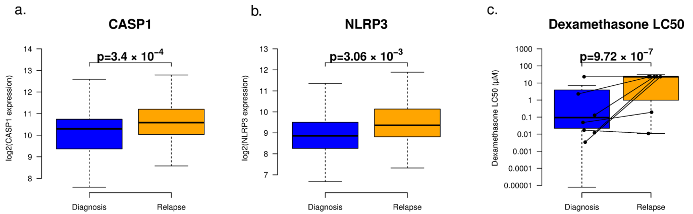
Figure 4. CASP1 and NLRP3 expression is higher and glucocorticoid resistance is greater in leukemia cells at the time of disease relapse
