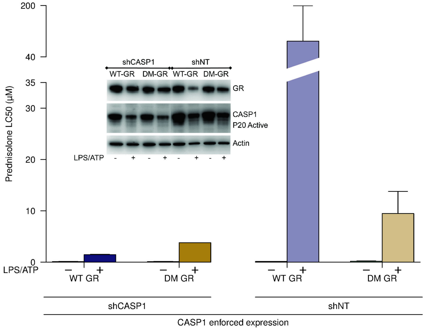
Figure 6. Expression of glucocorticoid receptor with both CASP1 cleavage sites mutated to AAAA mitigates CASP1 induced prednisolone resistance NALM-6 cells overexpressing CASP1 co-transfected with either non-targeting scrambled hairpin (shNT) or shRNA hairpins targeting CASP1 (shCASP1) were stably transduced with lentiviral vectors containing a wild-type glucocorticoid receptor or a glucocorticoid receptor in which both CASP1 cleavage sites had been eliminated (double mutagenized glucocorticoid receptor, DM-GR). The sensitivity (LC 50 ) of these cells to prednisolone was determined by MTT assays, revealing that cells overexpressing a glucocorticoid receptor without CASP1 cleavage sites remained sensitive to glucocorticoids when CASP1 was overexpressed. The inset is a western blot depicting recombinant glucocorticoid receptor protein levels (wild-type, or double mutagenized), in cells at time of MTT drug sensitivity assays. Data are representative of three independent experiments with standard deviation bars.
