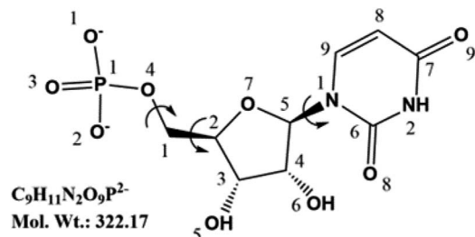
Fig. 1 Structure of UMP^{2-} with atomic numbering. Flexible torsion angles are indicated by \varphi_1 (C9–N1–C5–O7), \varphi_2 (C3–C2–C1–O4), and \varphi_3 (C2–C1–O4–P1).
