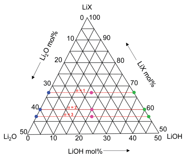
Fig. 1 Synthesized \text{LiX}(\text{Li}_{3-p}\text{OH}_p\text{X})_n compositions with \text{X} = \text{Br} and \text{Cl} , n = 1, 2, \text{ and } 3 , and p = 0, 0.5, \text{ and } 1 , presented in a ternary phase diagram.
