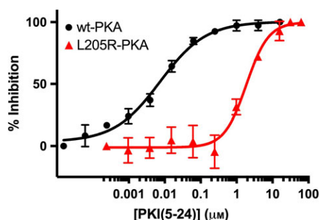
Fig. 4. Inhibition of wt-PKAC \alpha (black circles) and the L205R-PKAC \alpha mutant (red triangles) by PKI(5-24). The inhibitor concentration ranges for PKI(5-24) (this figure) and H89 (Fig. 5) are different.
