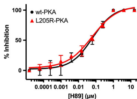
Fig. 5. Inhibition of wt-PKAC \alpha (black circles) and the L205R-PKAC \alpha mutant (red triangles) by H89. The inhibitor concentration ranges for PKI(5-24) (Fig. 4) and H89 (this figure) are different.
