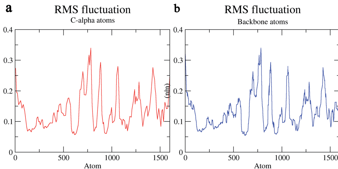
Fig. 8 RMSF ( \text{\AA} ) of (a) C atoms (b) protein backbone of 5/5I12 complex.
