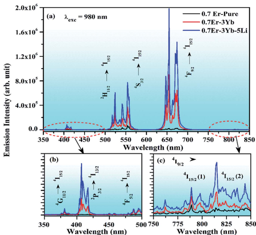
Fig. 12 (a) Comparison in UC emission intensity of 0.7\text{Er}^{3+} (pure), 0.7\text{Er}^{3+}/3\text{Yb}^{3+} , and 0.7\text{Er}^{3+}/3\text{Yb}^{3+}/\text{Li}^+ doped and co-doped \text{ZnGa}_2\text{O}_4 phosphors on excitation with 980 nm. Figures (b) and (c) are the UC emission spectra in the near UV-blue and NIR regions, respectively.
