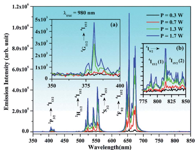
Fig. 11 Effect of incident pump power on the UC emission intensity of 0.7\text{Er}^{3+}/3\text{Yb}^{3+} co-doped \text{ZnGa}_2\text{O}_4 phosphor at 0.3, 0.7, 1.3, and 1.7 W. The inset (a) is the zoomed spectra in the near UV region whereas the inset (b) shows spectra in the NIR region, respectively.
