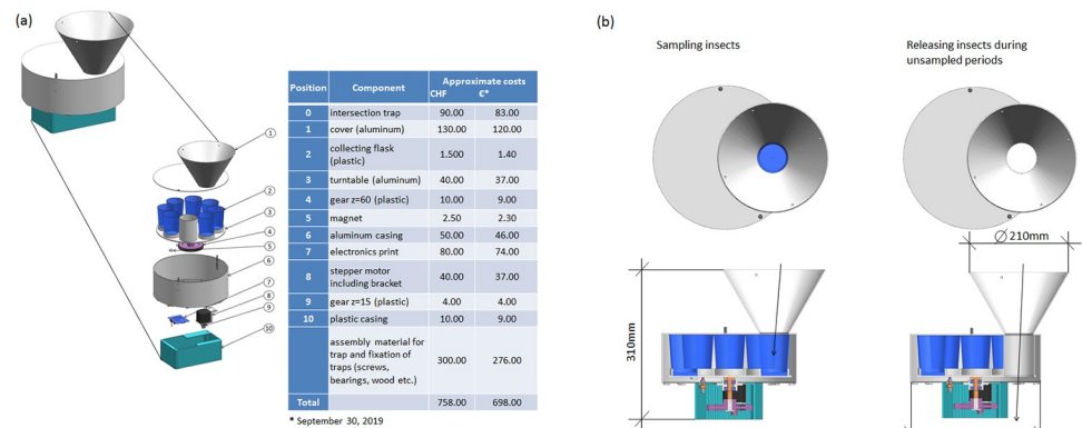
Fig 2. (a) Design and components of the turntable to optimize insect sampling including a list of required components and their approximate costs. Labor costs are not included; (b) position during periods of sampling (cups placed underneath the trap funnel) and non-sampling periods, when insects are released through the pass-through hole.
