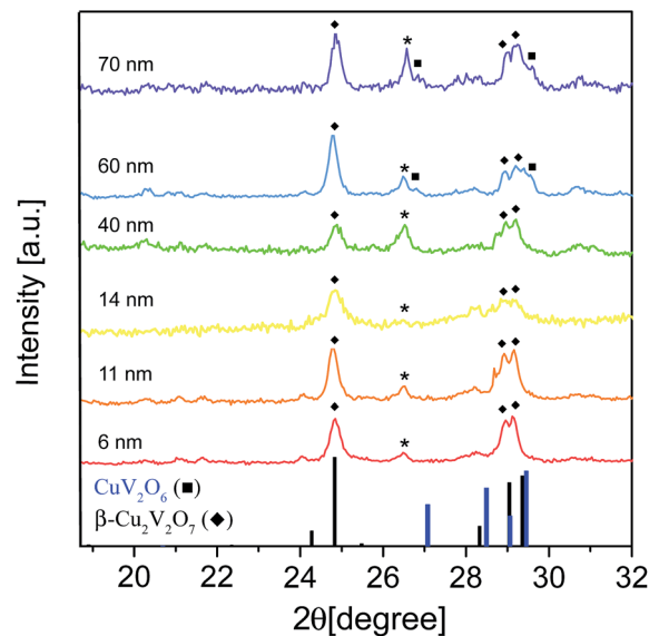
Fig. 3 XRD patterns of films synthesized from Cu NC seeds of 6 nm, 11 nm, 14 nm, 40 nm, 60 nm and 70 nm, reacted with \text{VO}(\text{acac})_2 and annealed at 350^\circ\text{C} for 8 hours. Monoclinic \beta\text{-Cu}_2\text{V}_2\text{O}_7 (PDF-01-076-2820) and triclinic \text{CuV}_2\text{O}_6 (PDF-00-045-1054) reference positions of the Bragg peaks are reported at the bottom. The asterisk symbol * indicates the peaks for \text{V}_2\text{O}_5 (PDF-00-041-1426).
