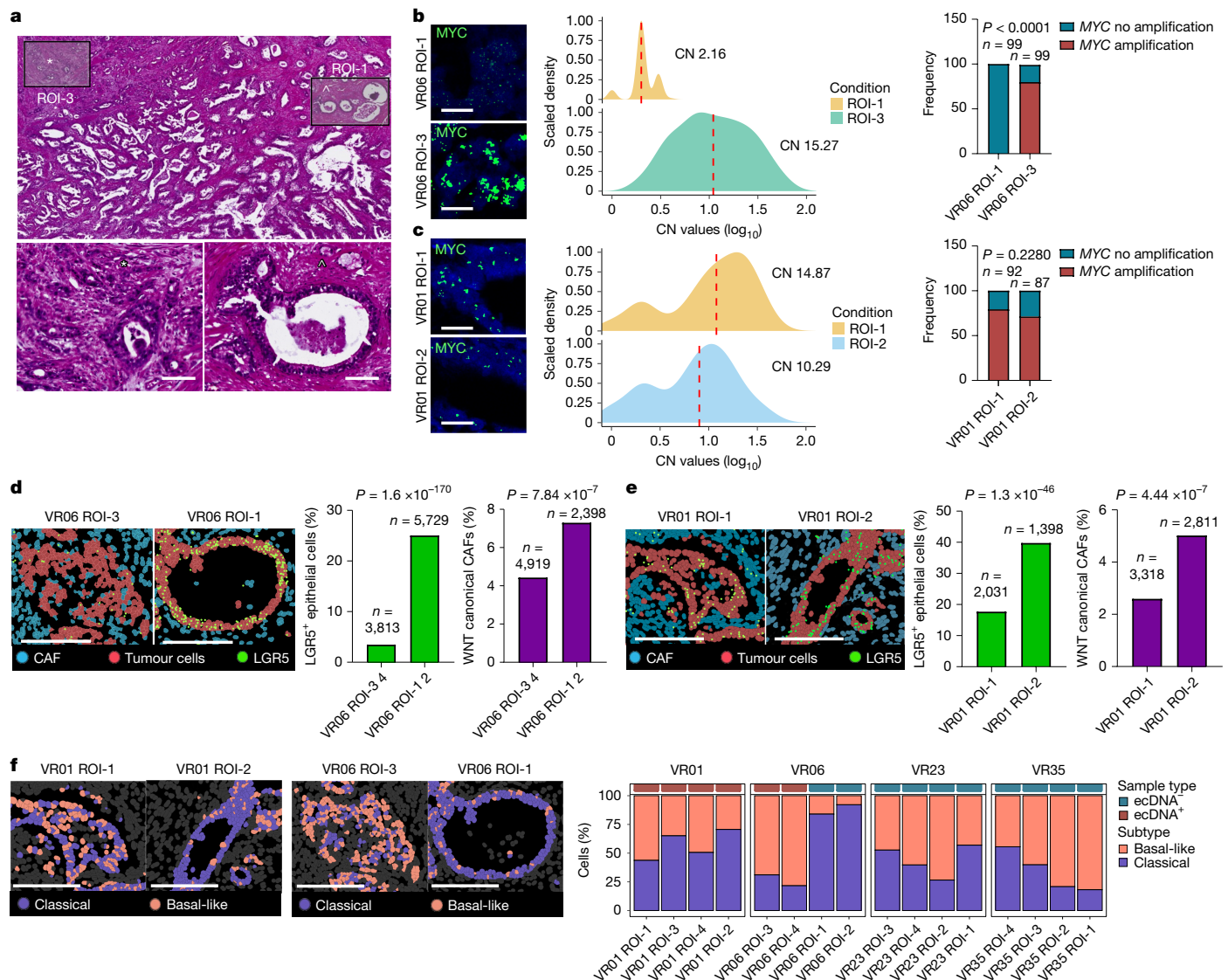
Fig. 5 | Spatial mapping of ecDNA-driven MYC amplifications and epithelial cell states. a , Post-Xenium haematoxylin and eosin of VR06-P (top). The magnifications of ROI-1 (caret; bottom right) and ROI-3 (asterisk; bottom left) demonstrate the different morphology of the neoplastic epithelium. Scale bars, 100 \mu m. b , Interphase FISH of ROI-1 and ROI-3 from VR06-P (left). Scale bars, 20 \mu m. Distribution of MYC copy number (CN) states per nucleus with indication of the average MYC copy number per ROI (middle). The dashed red line indicates the median copy number state. In the two selected ROIs, the proportion of nuclei (ROI-1 n = 99 and ROI-3 n = 99 ) with MYC amplification (defined as copy number > 5 ) is shown (right). The P value was calculated using Fisher's exact two-sided test. c , Interphase FISH of ROI-1 and ROI-2 from VR01-P (left). Scale bars, 20 \mu m. Distribution of MYC copy number states per nucleus with indication of the average MYC copy number per ROI (middle). The dashed
