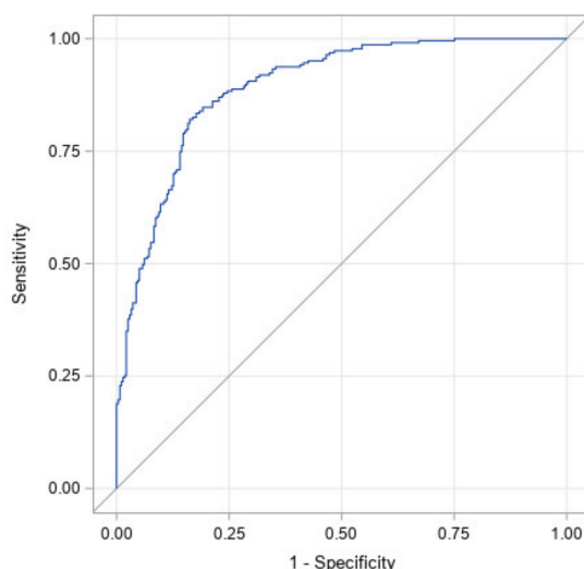
Figure 3. Receiver operating characteristic (ROC) curve for a model with all factors. Factors are: initial cephalic index (CI), initial cranial vault asymmetry index (CVAI), interaction between initial CI and CVAI, initial age, prematurity, and torticollis). The area under the curve is 0.89.
